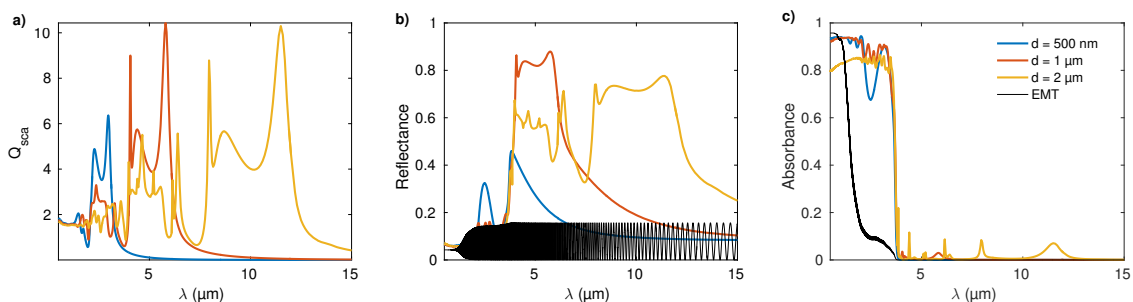
Figure 1: Scattering efficiency Q_{sca} of Te particles of different diameters (a), spectral reflectance and absorbance (b-c) for composites with Te inclusions in a host medium of refractive index n_m = 1.5 , thickness l = 200 \mu\text{m} and volume fraction of inclusions f = 0.01 .
